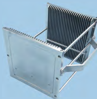
6吋不锈钢晶舟盒 6 Inch Stainless Steel Process Cassettes
