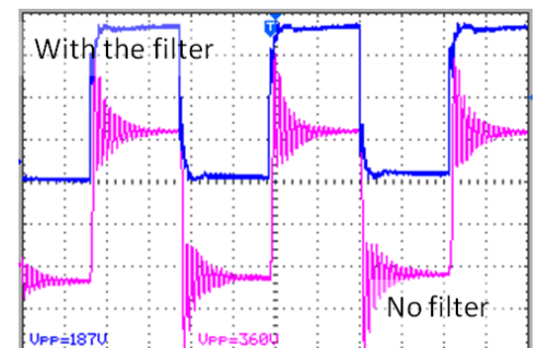
Drive Waveform: No More Ringing
