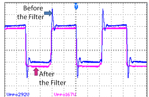
Drive Waveform: No More Overvoltage
